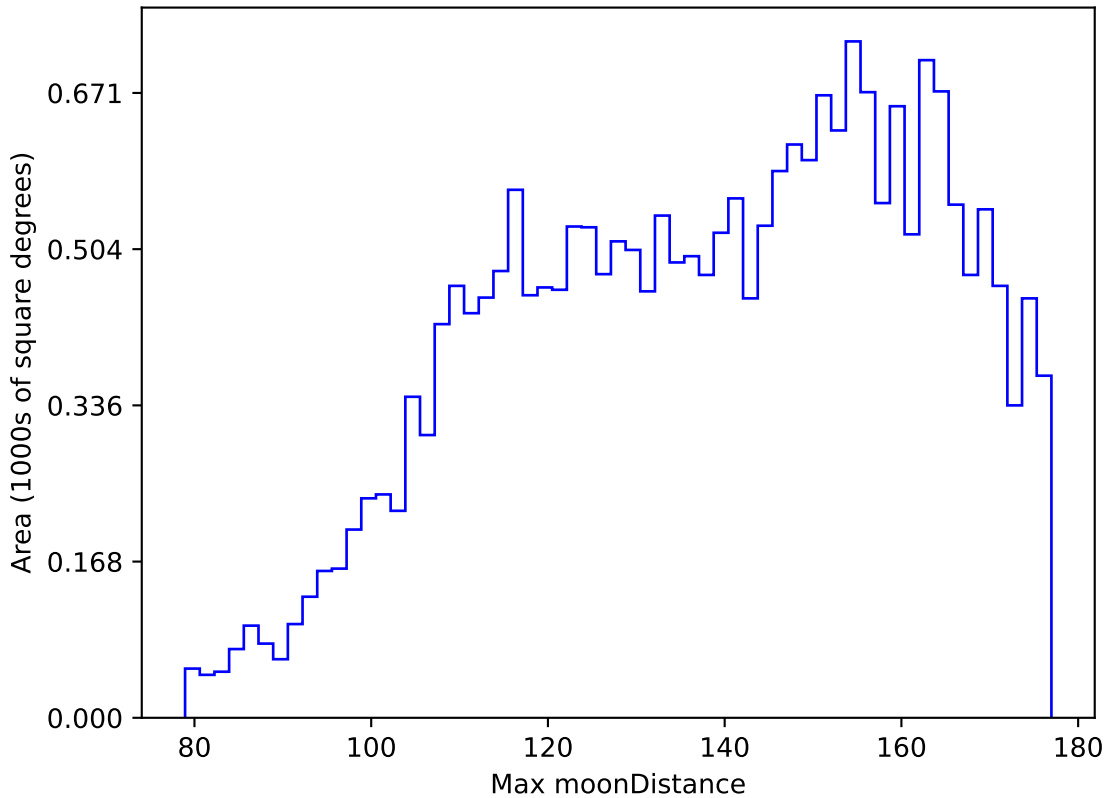
too_elab_r64_d3_griz_v3.4_10yrs All sky y band: Max moonDistance
