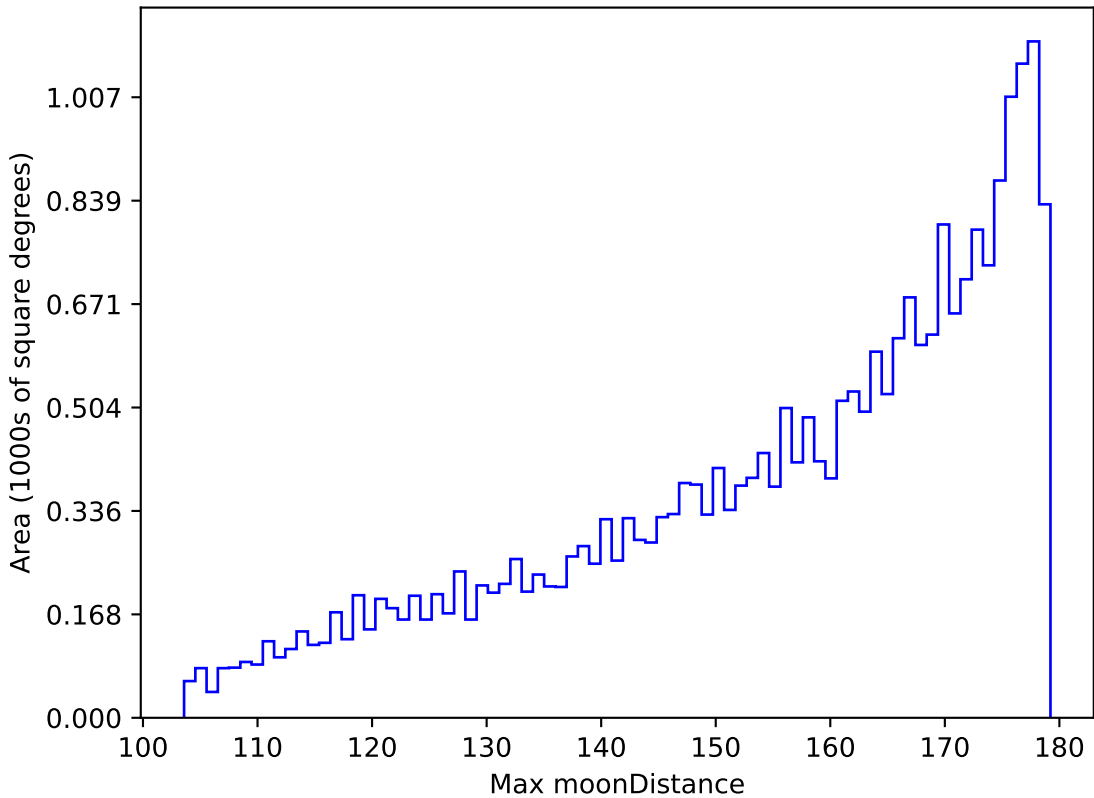
too_elab_r64_d3_griz_v3.4_10yrs All sky i band: Max moonDistance
