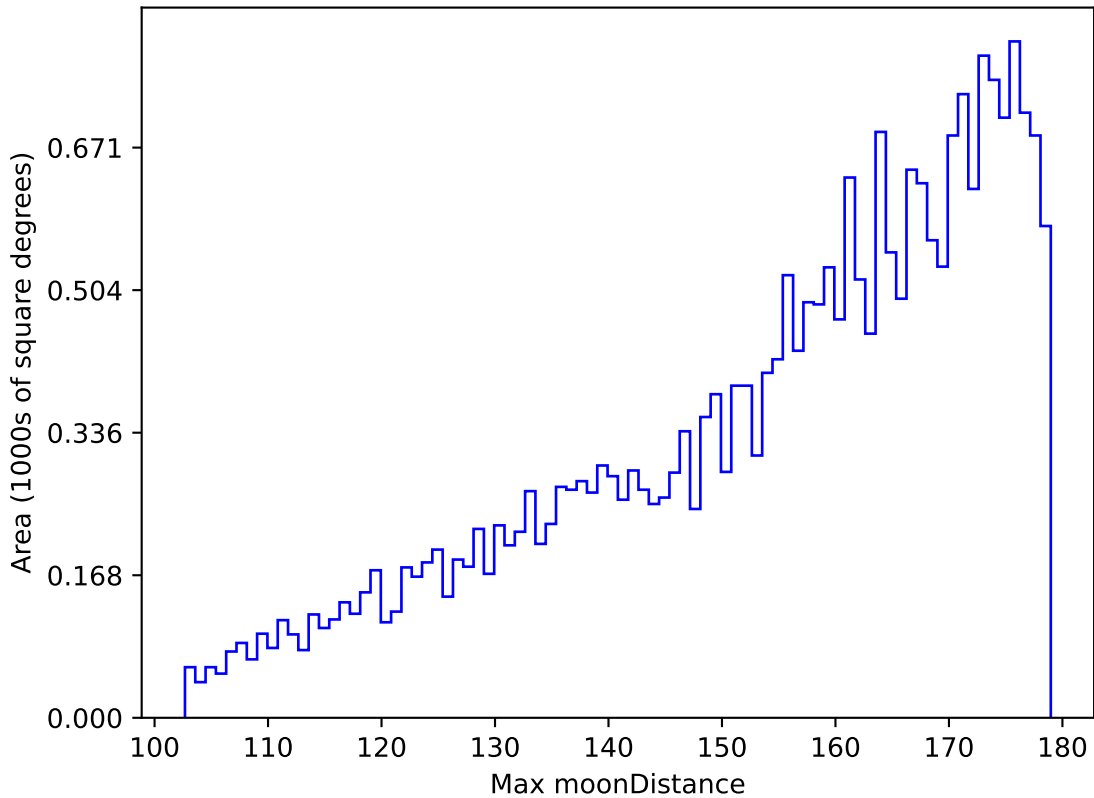
too_elab_r64_d3_griz_v3.4_10yrs All sky g band: Max moonDistance
