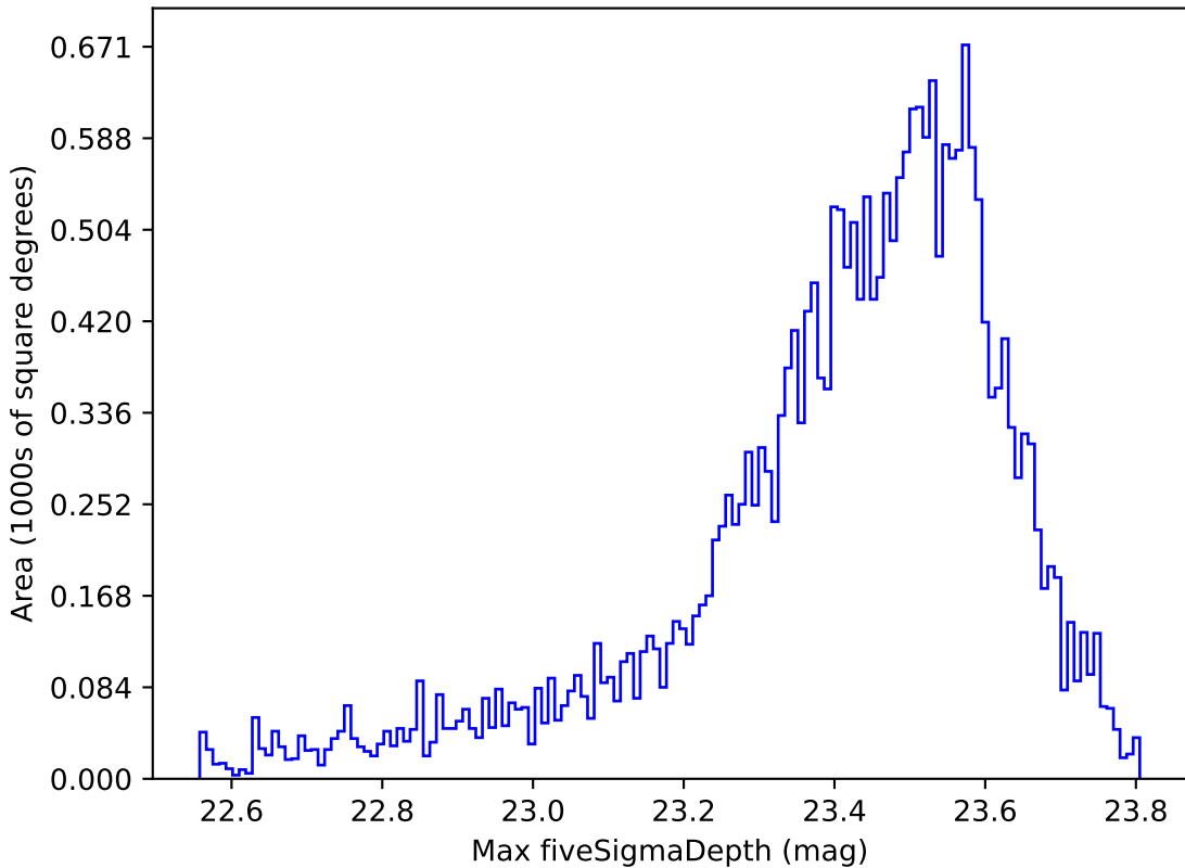
too_elab_r64_d3_griz_v3.4_10yrs Yr 1 z band: Max fiveSigmaDepth
