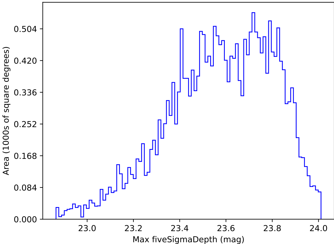
too_elab_r64_d3_griz_v3.4_10yrs Yr 1 u band: Max fiveSigmaDepth
