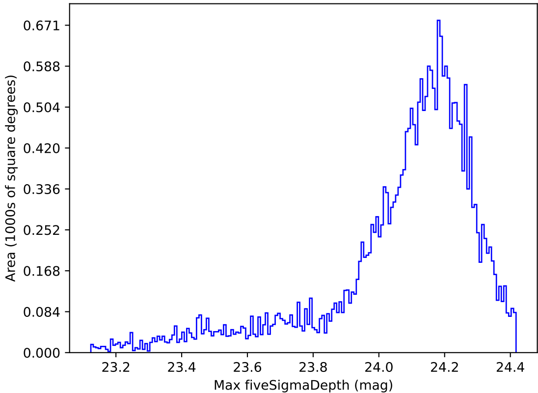
too_elab_r64_d3_griz_v3.4_10yrs Yr 1 i band: Max fiveSigmaDepth
