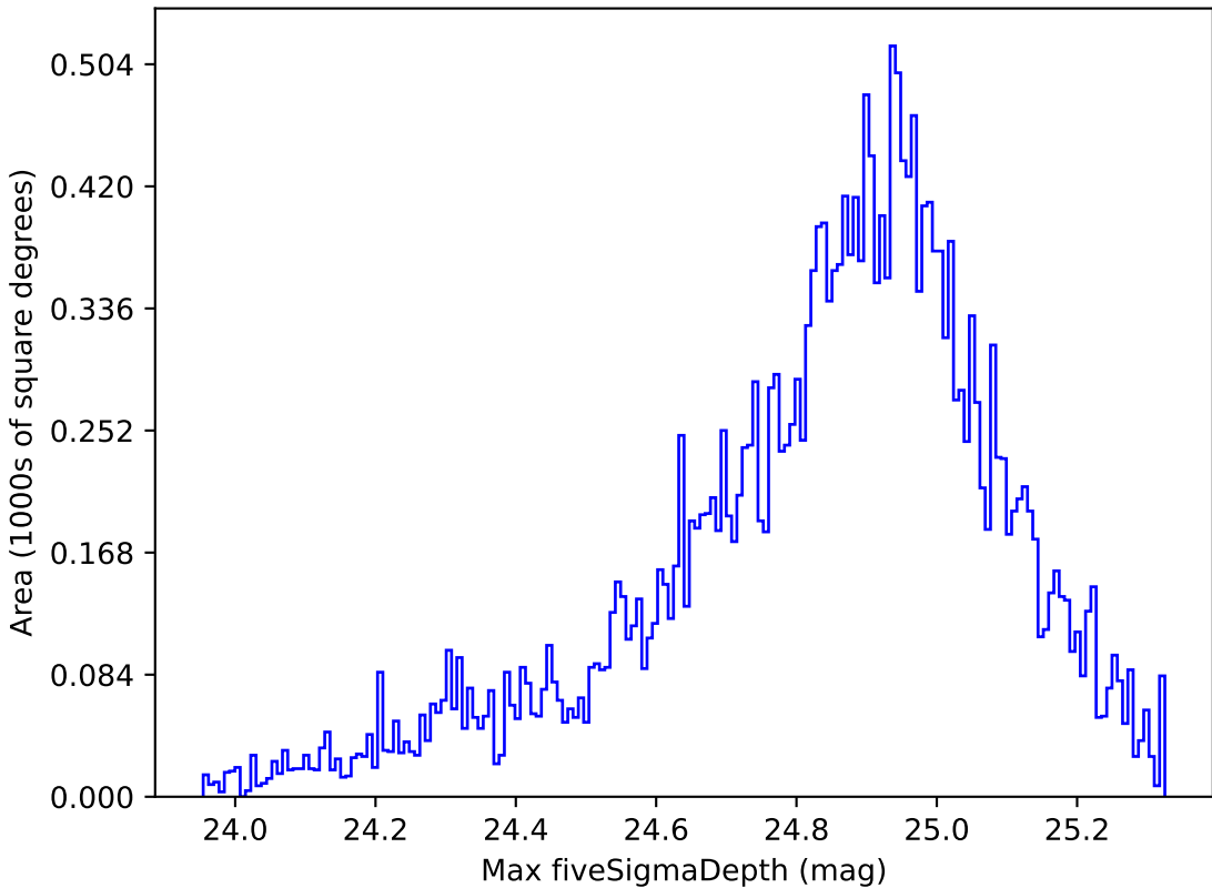
too_elab_r64_d3_griz_v3.4_10yrs Yr 1 g band: Max fiveSigmaDepth
