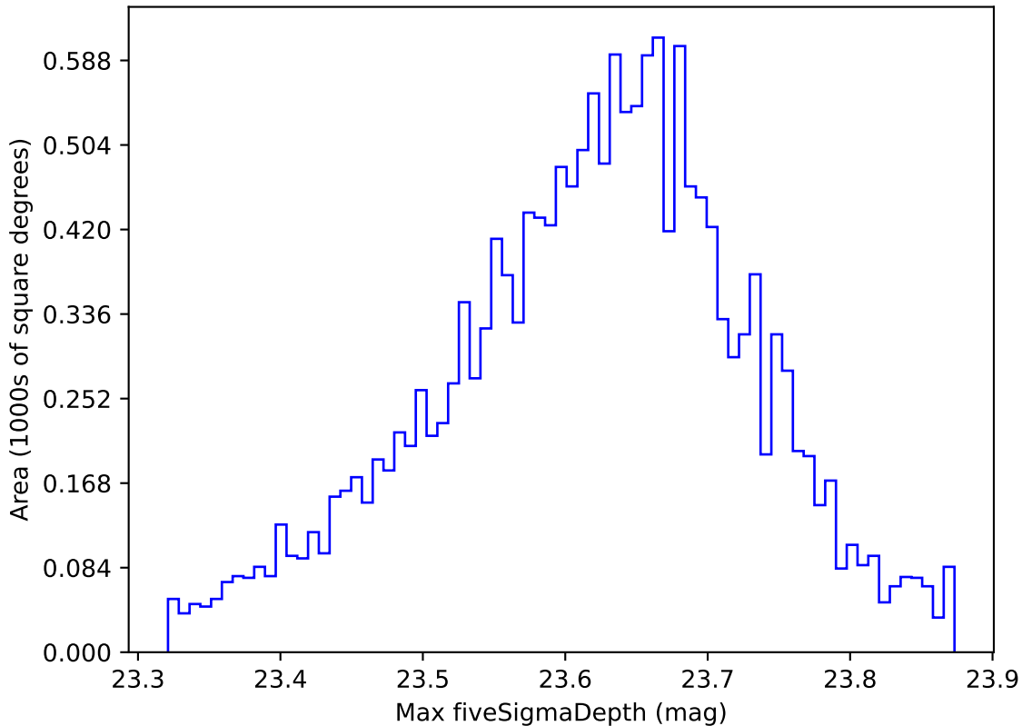
too_elab_r64_d3_griz_v3.4_10yrs WFD z band: Max fiveSigmaDepth
