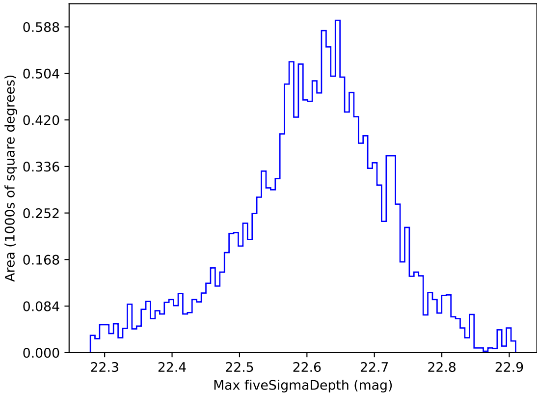
too_elab_r64_d3_griz_v3.4_10yrs WFD y band: Max fiveSigmaDepth
