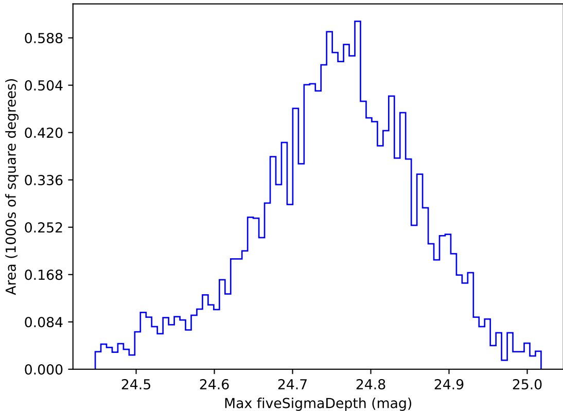
too_elab_r64_d3_griz_v3.4_10yrs WFD r band: Max fiveSigmaDepth
