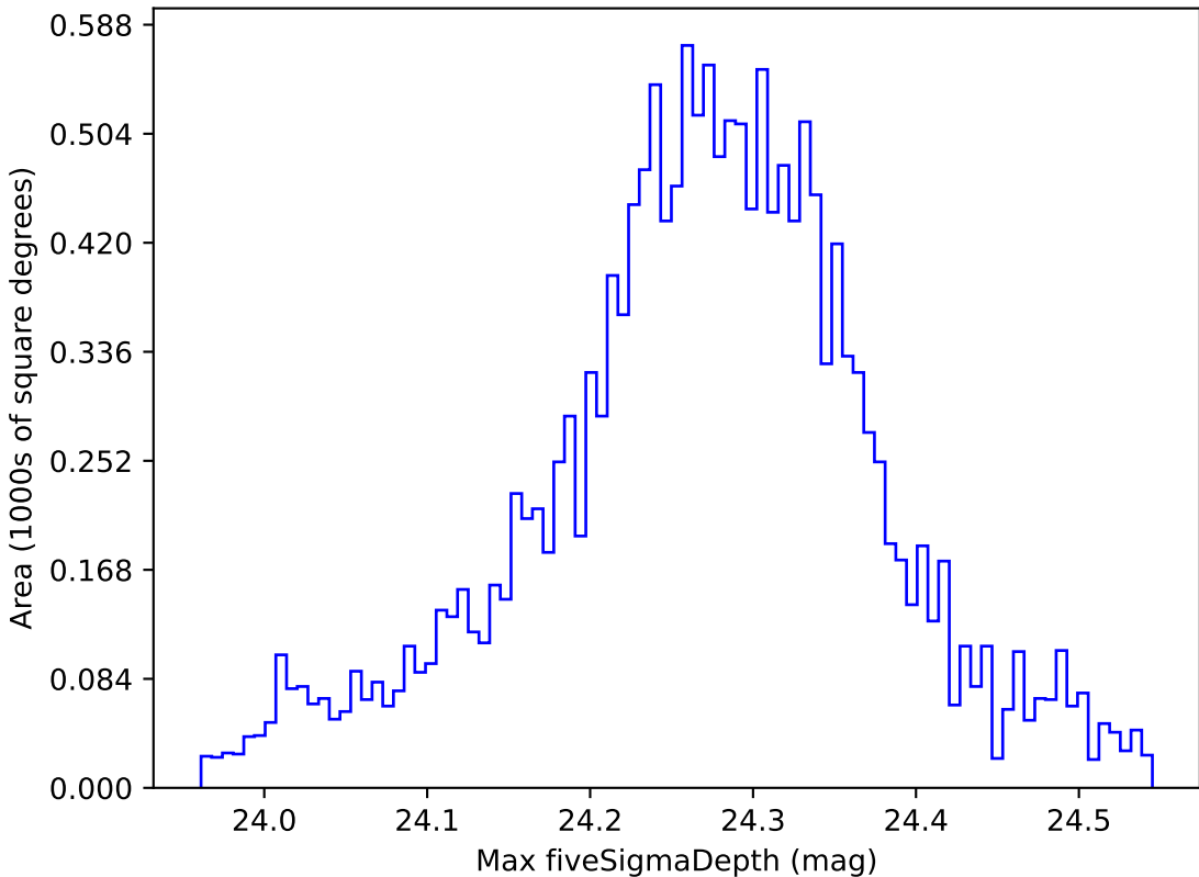
too_elab_r64_d3_griz_v3.4_10yrs WFD i band: Max fiveSigmaDepth
