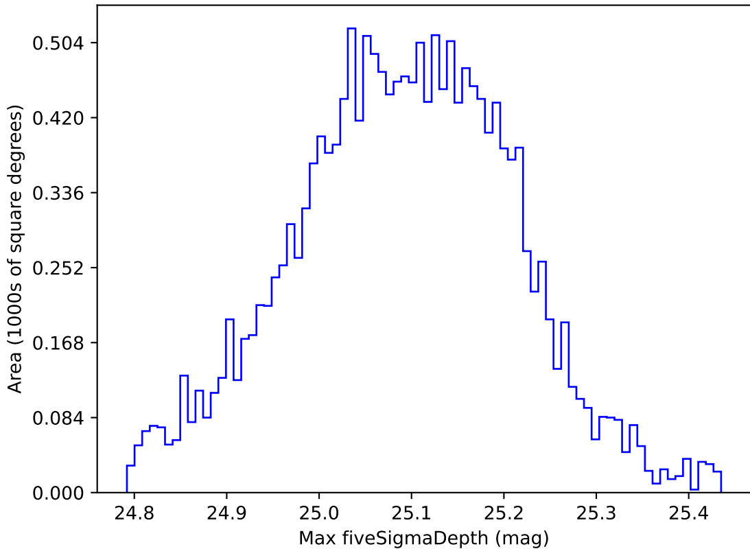
too_elab_r64_d3_griz_v3.4_10yrs WFD g band: Max fiveSigmaDepth
