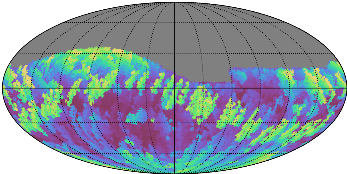
too_elab_r64_d3_griz_v3.4_10yrs Yr 1 r band: Max airmass
