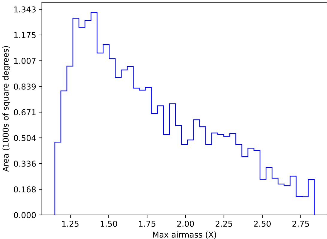
too_elab_r64_d3_griz_v3.4_10yrs Yr 1 i band: Max airmass
