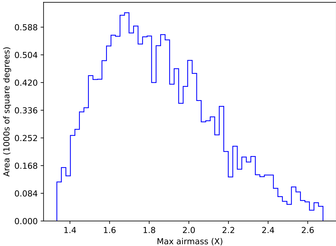
too_elab_r64_d3_griz_v3.4_10yrs WFD u band: Max airmass
