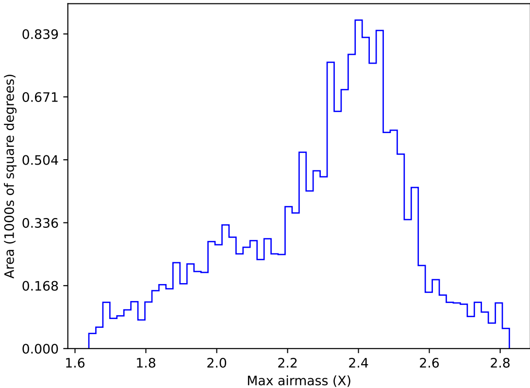
too_elab_r64_d3_griz_v3.4_10yrs WFD r band: Max airmass
