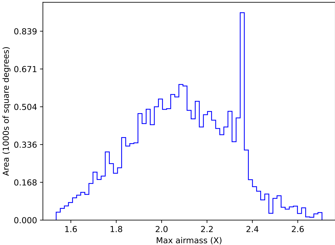
too_elab_r64_d3_griz_v3.4_10yrs WFD g band: Max airmass
