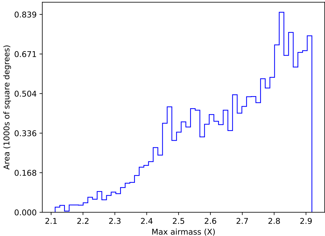
too_elab_r64_d3_griz_v3.4_10yrs WFD all bands: Max airmass
