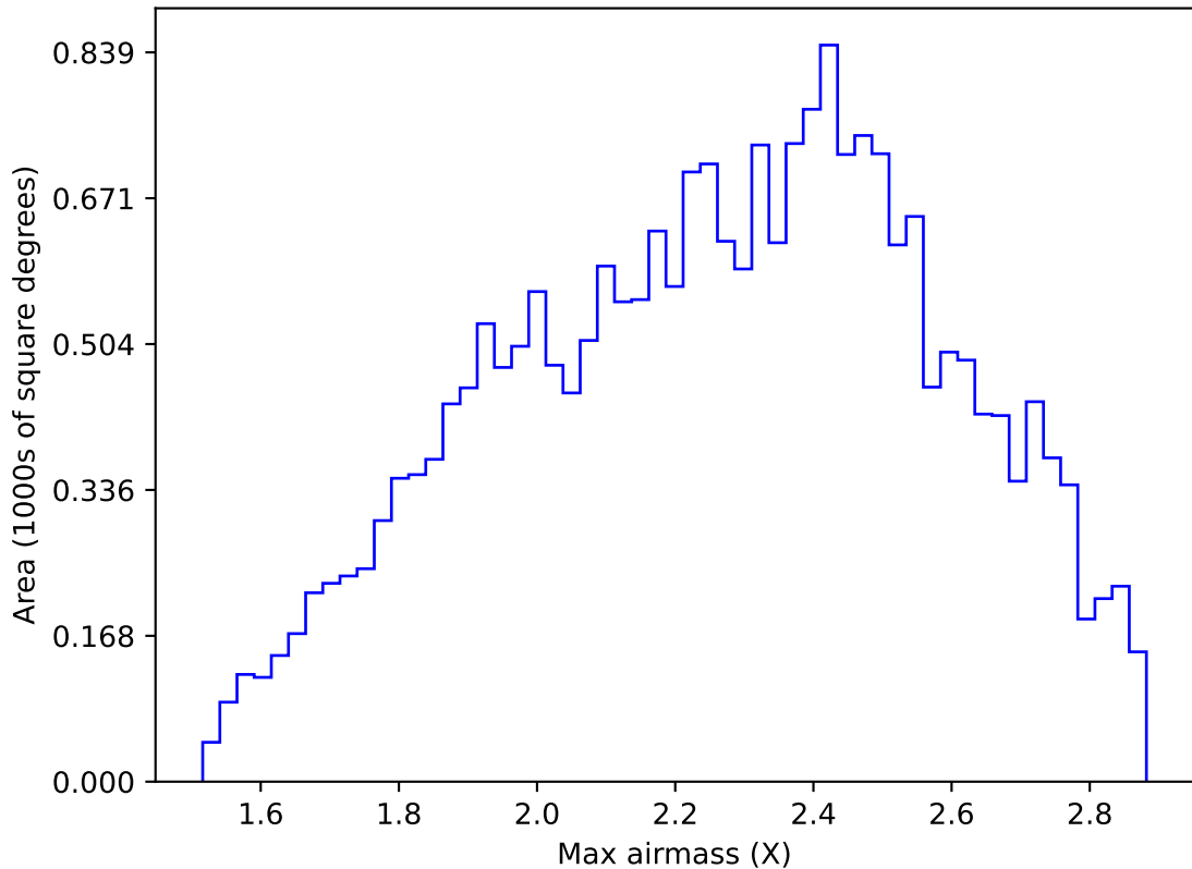
too_elab_r64_d3_griz_v3.4_10yrs All sky y band: Max airmass
