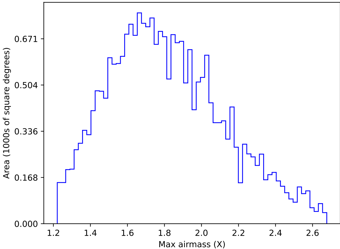
too_elab_r64_d3_griz_v3.4_10yrs All sky u band: Max airmass
