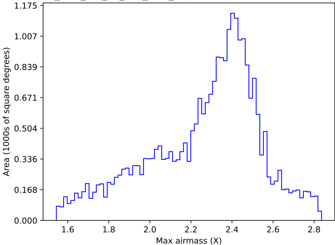
too_elab_r64_d3_griz_v3.4_10yrs All sky r band: Max airmass
