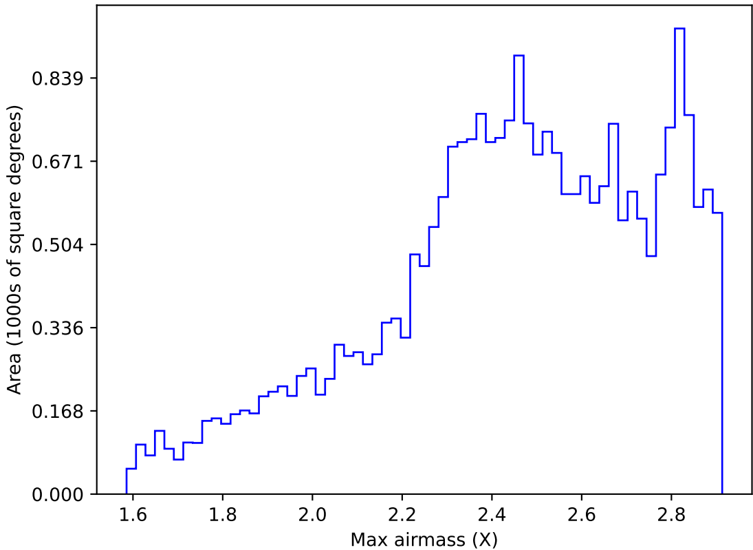
too_elab_r64_d3_griz_v3.4_10yrs All sky i band: Max airmass
