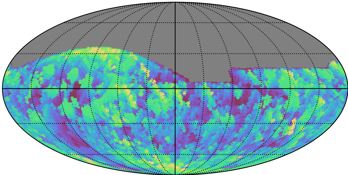
too_elab_r64_d3_griz_v3.4_10yrs All sky g band: Max airmass
