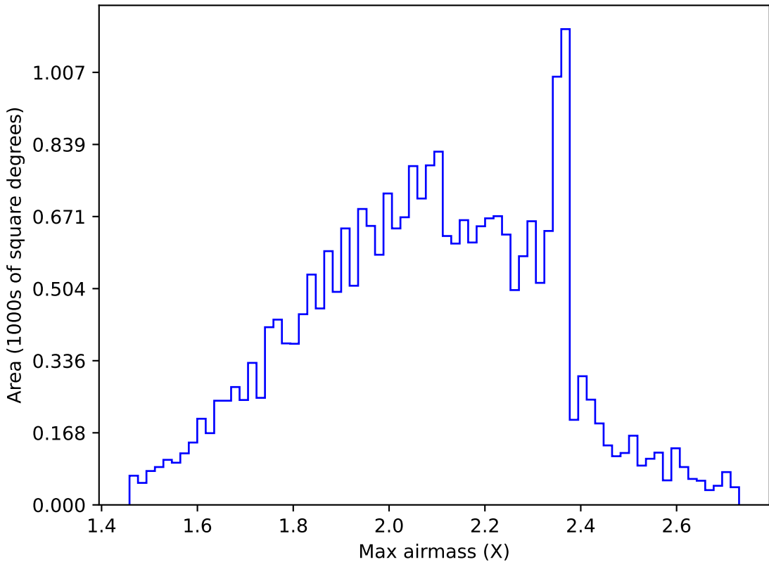
too_elab_r64_d3_griz_v3.4_10yrs All sky g band: Max airmass
