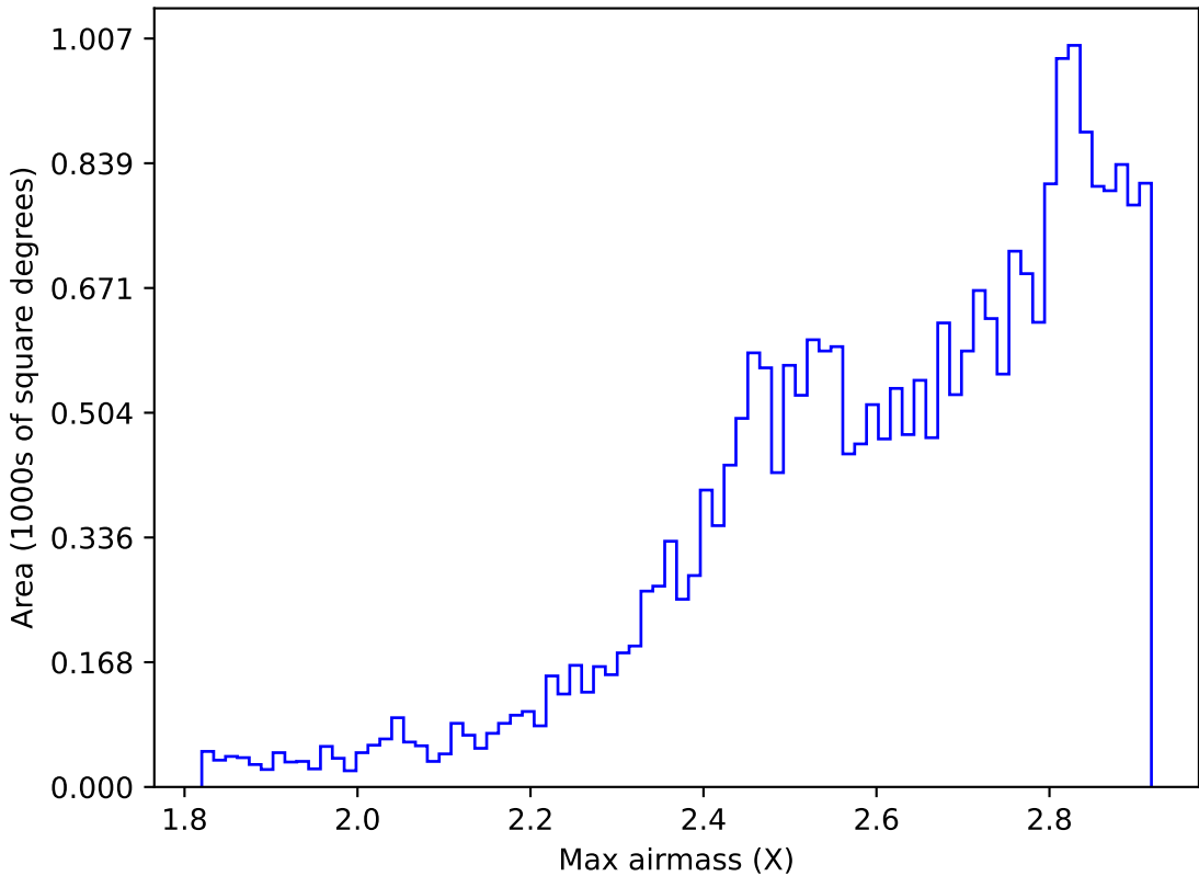
too_elab_r64_d3_griz_v3.4_10yrs All sky all bands: Max airmass
