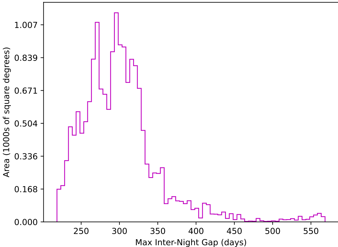
too_elab_r64_d3_griz_v3.4_10yrs WFD z band: Max Inter-Night Gap
