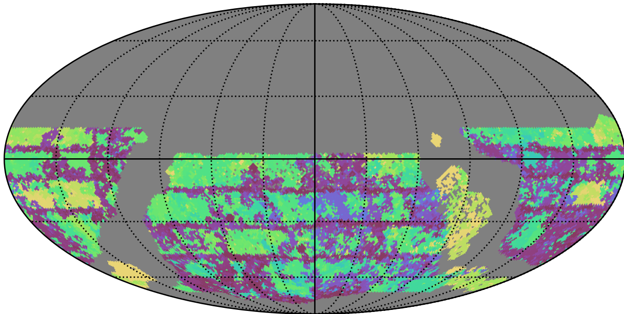
too_elab_r64_d3_griz_v3.4_10yrs WFD u band: Max Inter-Night Gap
