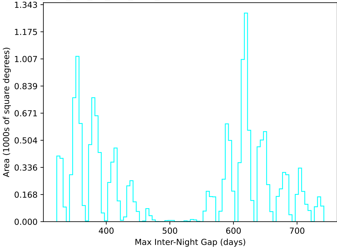
too_elab_r64_d3_griz_v3.4_10yrs WFD u band: Max Inter-Night Gap
