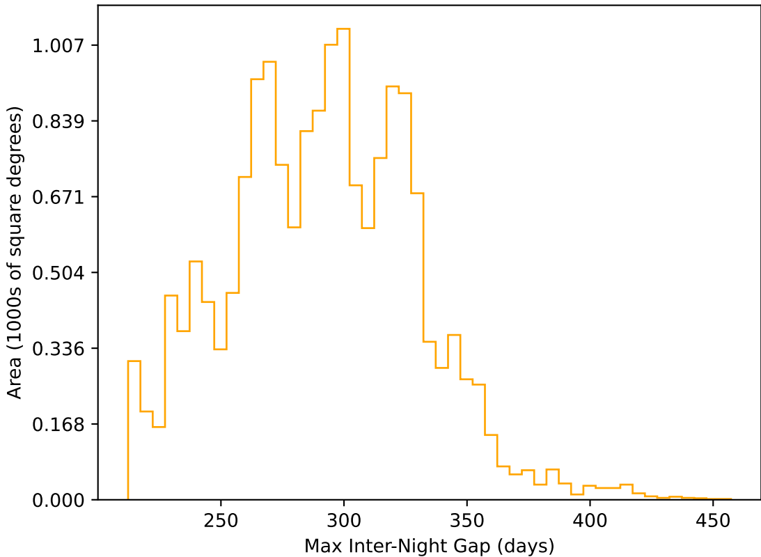
too_elab_r64_d3_griz_v3.4_10yrs WFD r band: Max Inter-Night Gap
