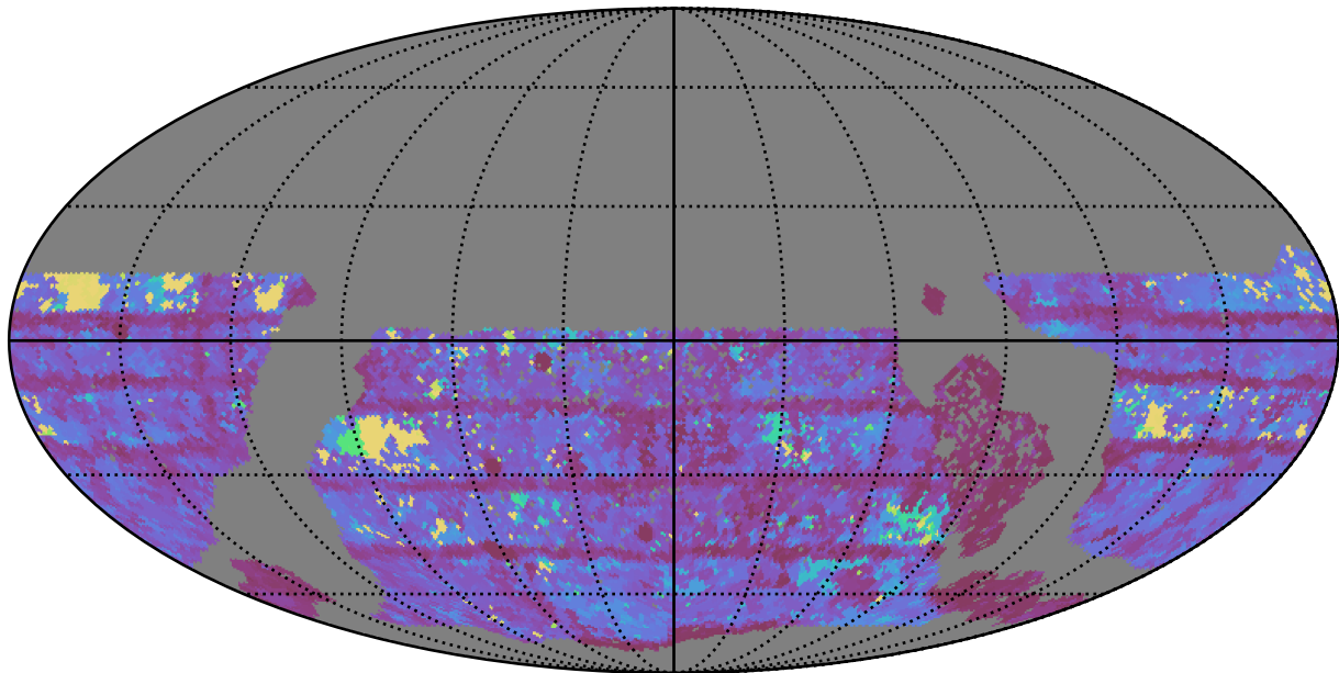
too_elab_r64_d3_griz_v3.4_10yrs WFD i band: Max Inter-Night Gap
