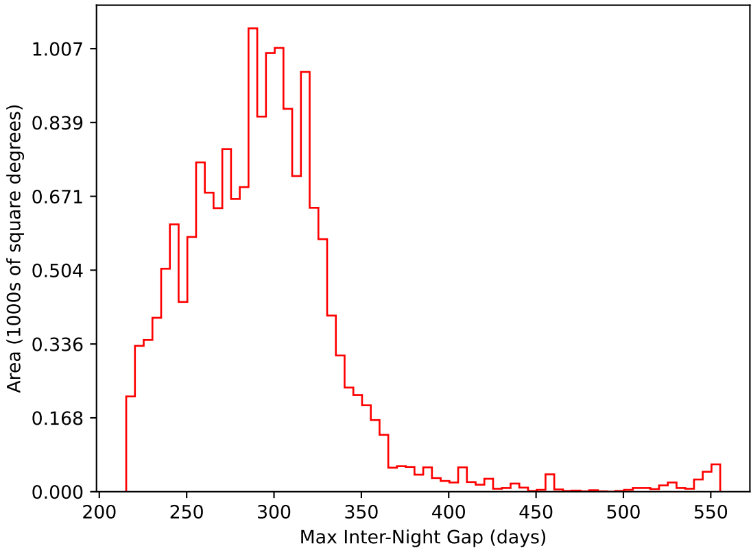
too_elab_r64_d3_griz_v3.4_10yrs WFD i band: Max Inter-Night Gap
