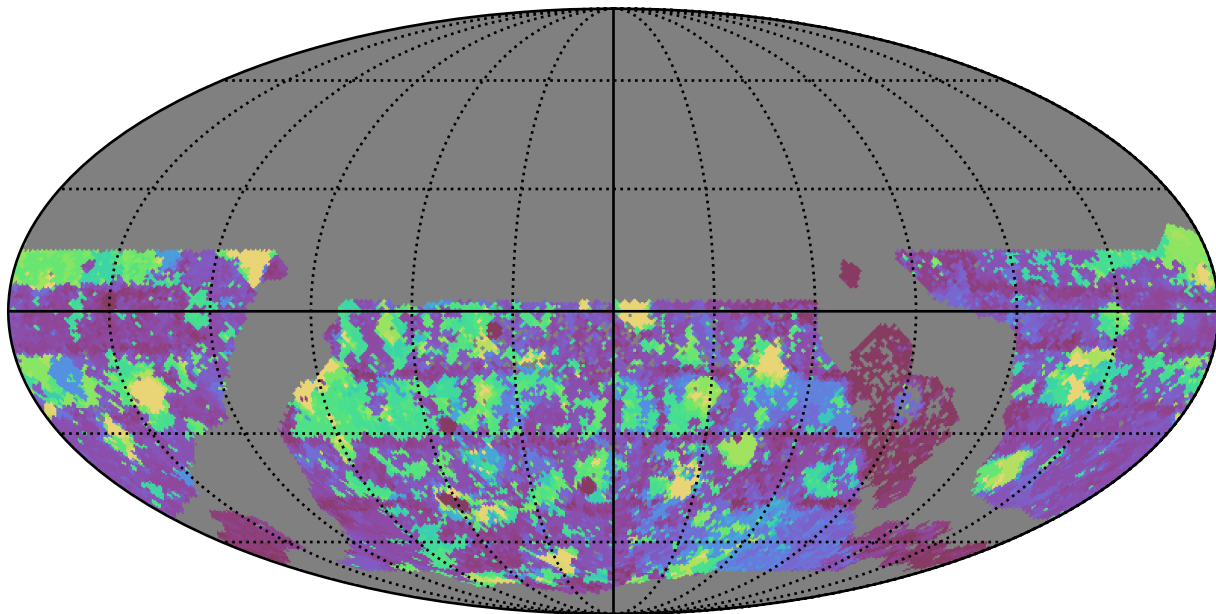
too_elab_r64_d3_griz_v3.4_10yrs WFD g band: Max Inter-Night Gap
