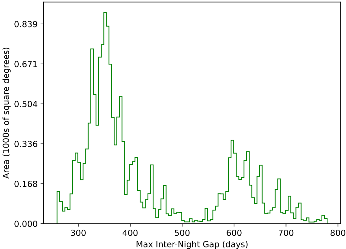
too_elab_r64_d3_griz_v3.4_10yrs WFD g band: Max Inter-Night Gap
