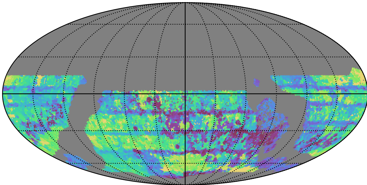
too_elab_r64_d3_griz_v3.4_10yrs WFD all bands: Max Inter-Night Gap
