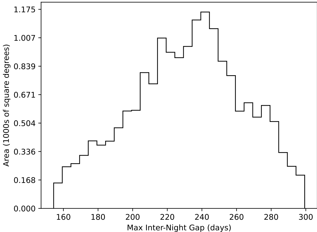
too_elab_r64_d3_griz_v3.4_10yrs WFD all bands: Max Inter-Night Gap
