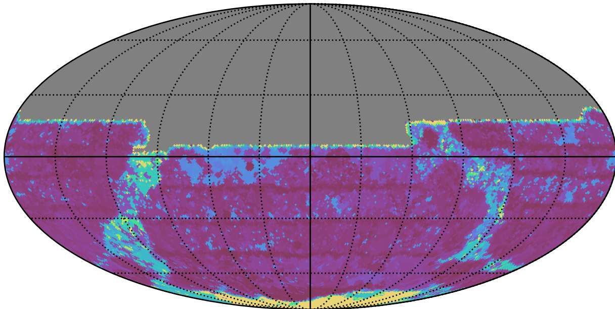
too_elab_r64_d3_griz_v3.4_10yrs All sky y band: Max Inter-Night Gap
