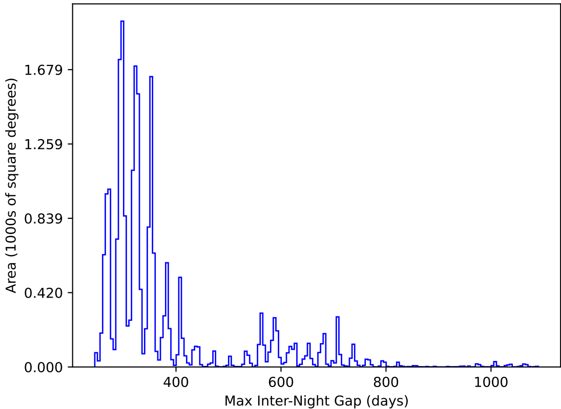
too_elab_r64_d3_griz_v3.4_10yrs All sky y band: Max Inter-Night Gap
