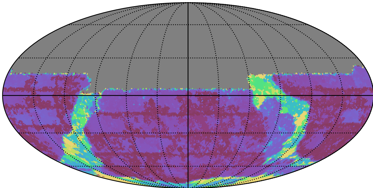
too_elab_r64_d3_griz_v3.4_10yrs All sky u band: Max Inter-Night Gap
