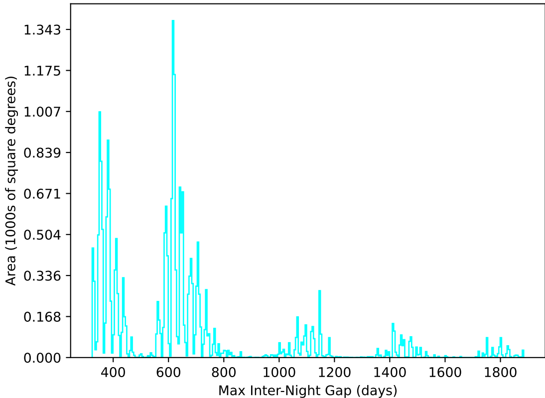
too_elab_r64_d3_griz_v3.4_10yrs All sky u band: Max Inter-Night Gap
