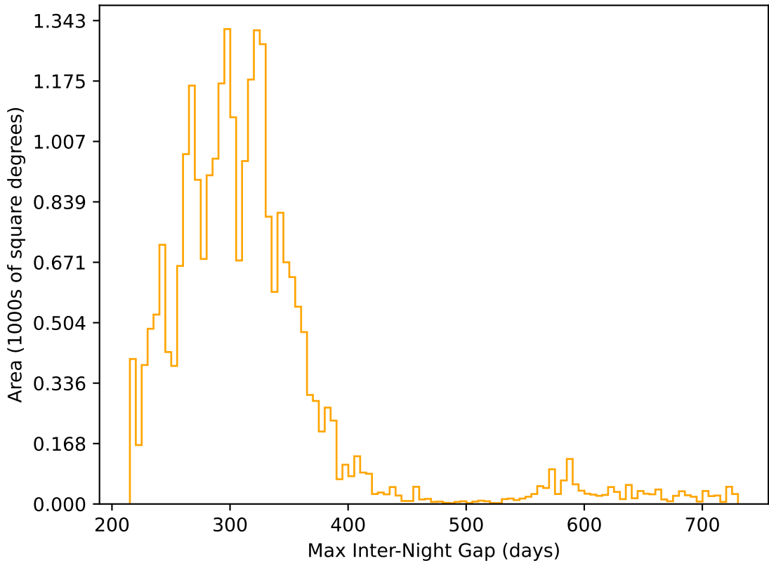
too_elab_r64_d3_griz_v3.4_10yrs All sky r band: Max Inter-Night Gap
