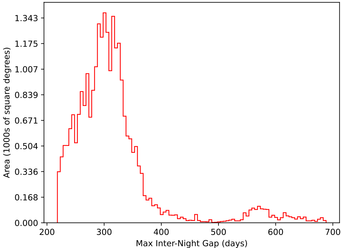
too_elab_r64_d3_griz_v3.4_10yrs All sky i band: Max Inter-Night Gap
