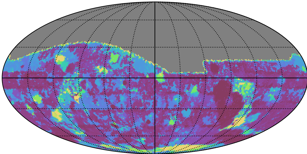
too_elab_r64_d3_griz_v3.4_10yrs All sky g band: Max Inter-Night Gap
