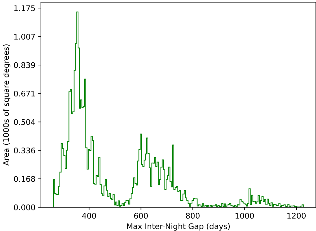
too_elab_r64_d3_griz_v3.4_10yrs All sky g band: Max Inter-Night Gap
