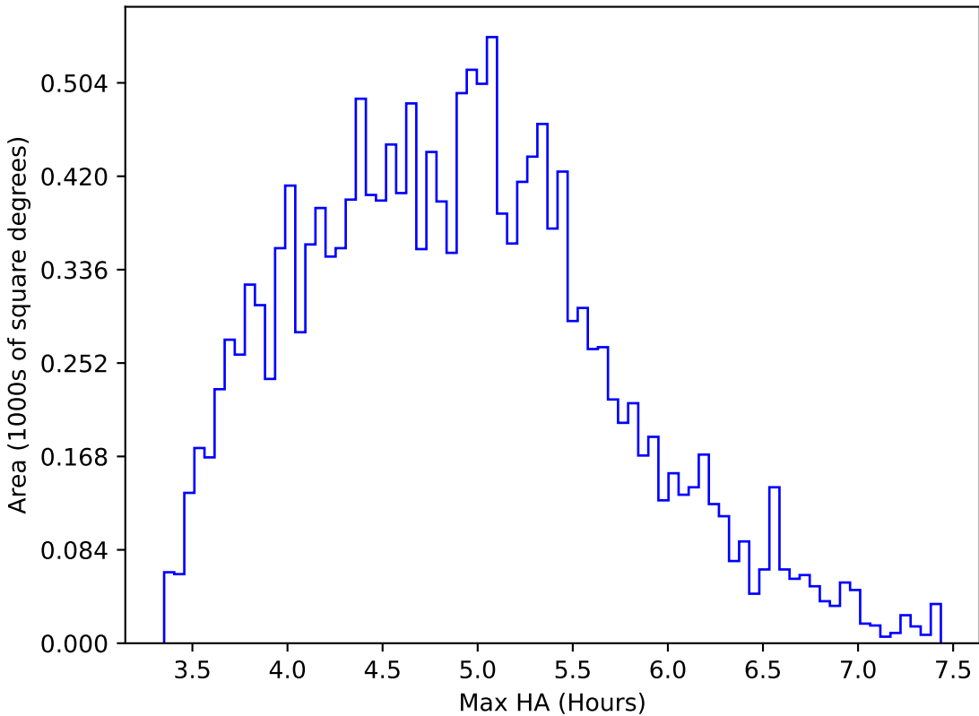
too_elab_r64_d3_griz_v3.4_10yrs WFD z band: Max HA
