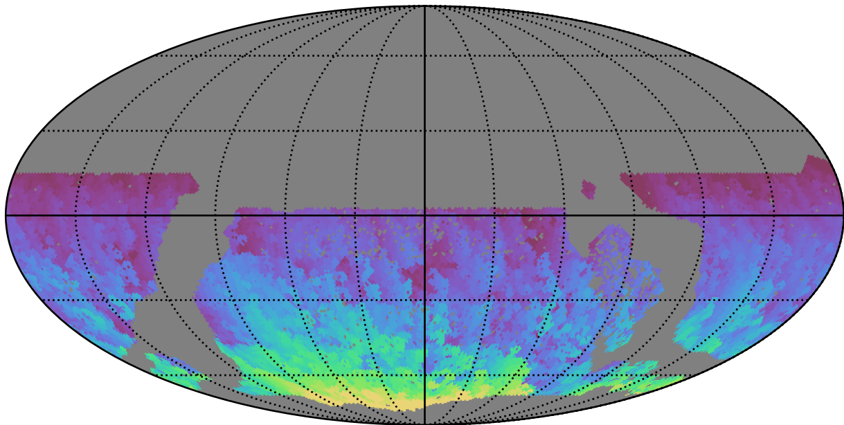
too_elab_r64_d3_griz_v3.4_10yrs WFD y band: Max HA
