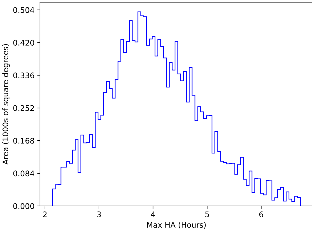
too_elab_r64_d3_griz_v3.4_10yrs WFD u band: Max HA
