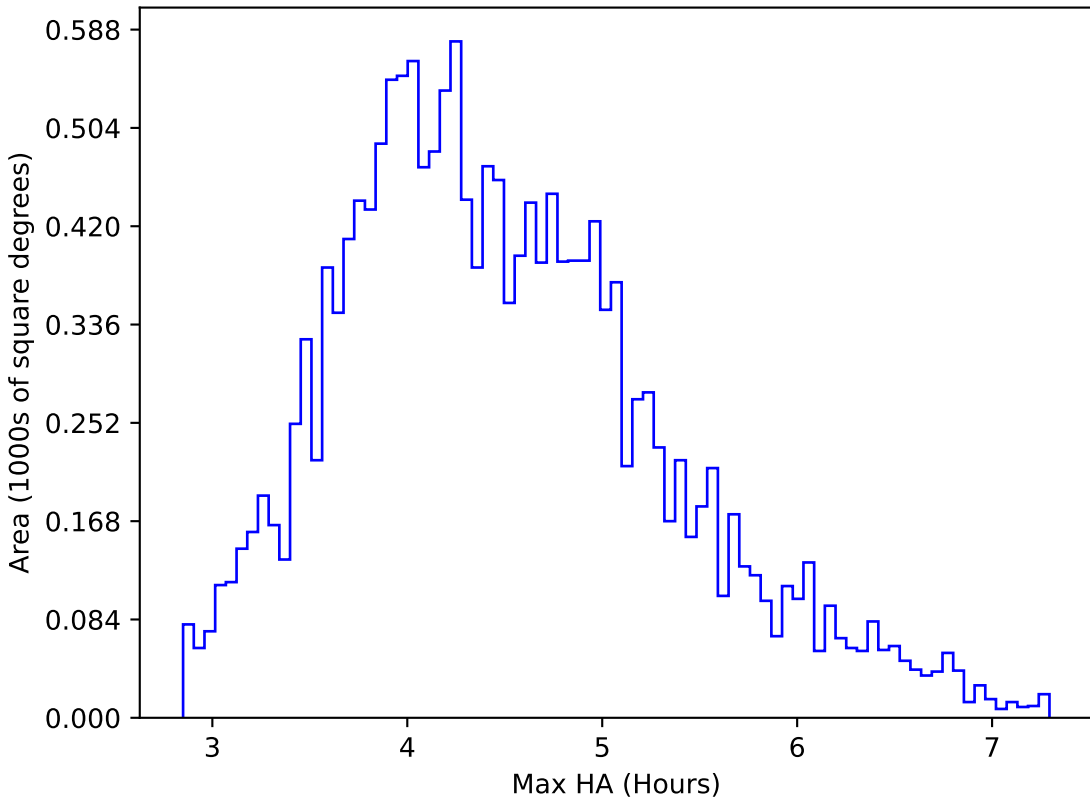
too_elab_r64_d3_griz_v3.4_10yrs WFD r band: Max HA
