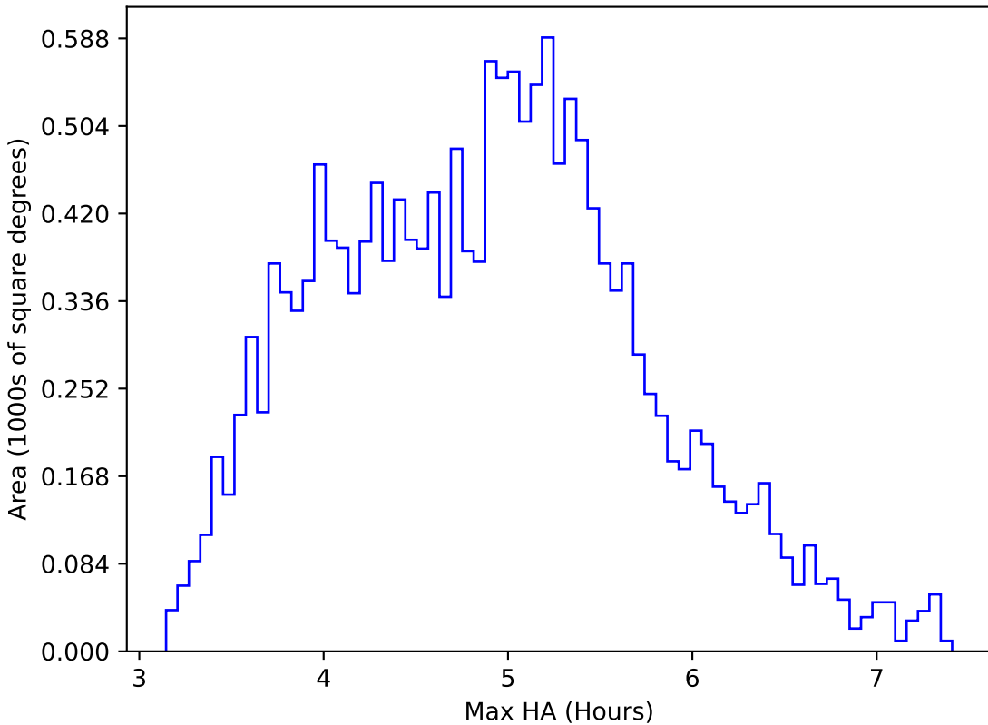
too_elab_r64_d3_griz_v3.4_10yrs WFD i band: Max HA
