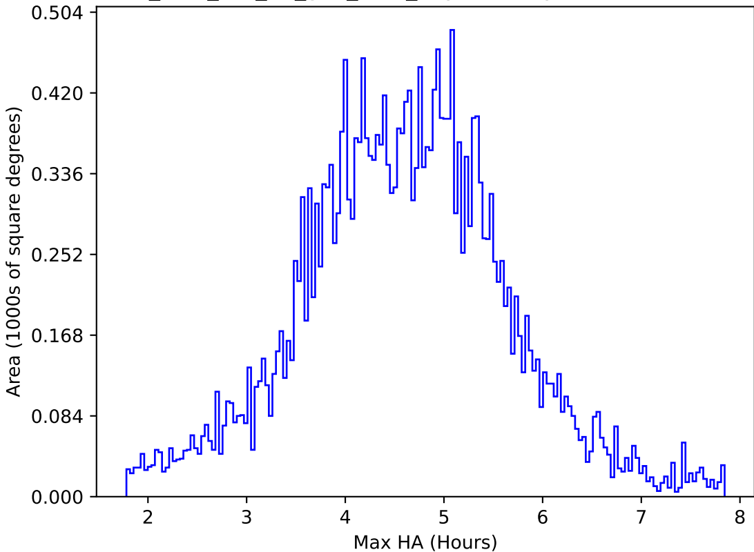
too_elab_r64_d3_griz_v3.4_10yrs All sky z band: Max HA
