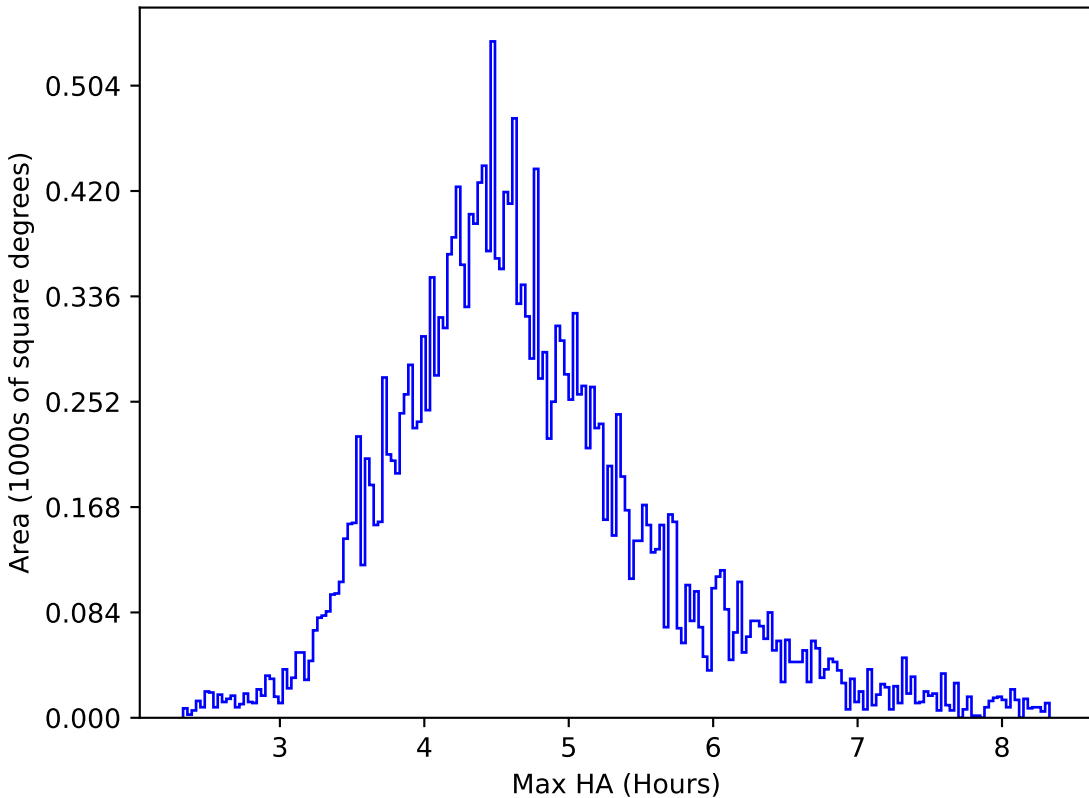
too_elab_r64_d3_griz_v3.4_10yrs All sky y band: Max HA
